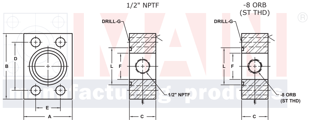
Model 6295 / 6296
